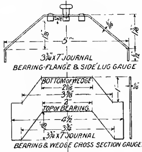
BEARING & WEDGE CROSS SECTION GAUGE.
